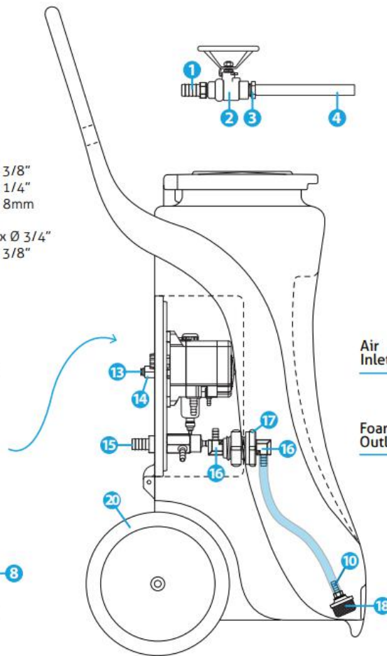
Cover - Internal View
